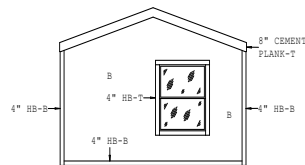
FRONT ELEVATION
