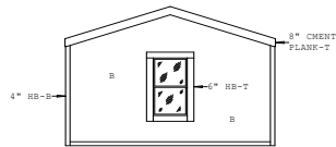
FRONT ELEVATION
