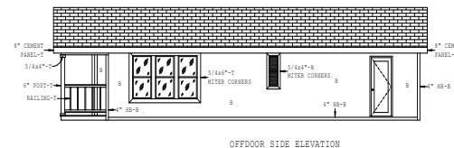
OUTDOOR SIDE ELEVATION
