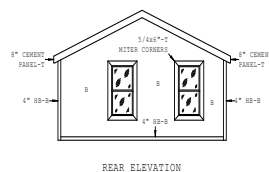
REAR ELEVATION
