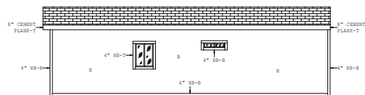
OFFDOOR SIDE ELEVATION
