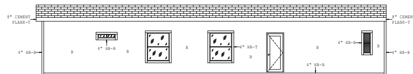
OFFDOOR SIDE ELEVATION
